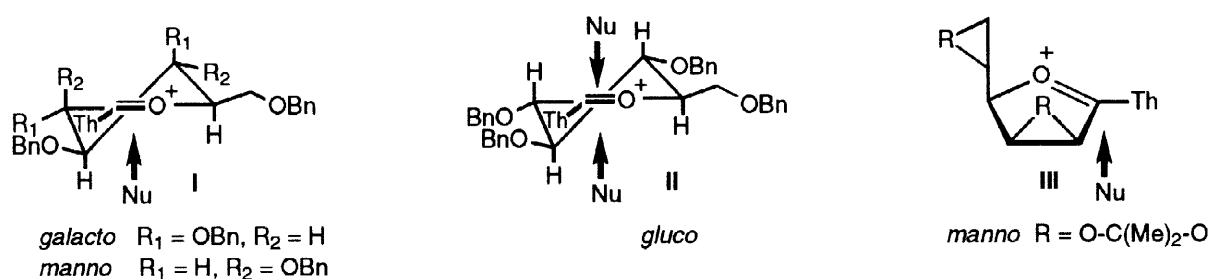
Figure 2. Stereochemical models for the reaction of thiazoly ketol acetates 1 with \text{P}(\text{OEt})_3 .
