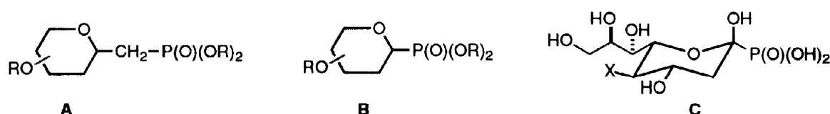
Figure 1. Glycosylphosphonate analogs of glycosylphosphates and sialic acids.
